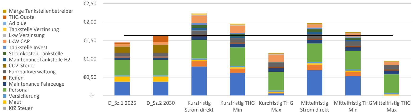
Logistikkosten [€/km]
